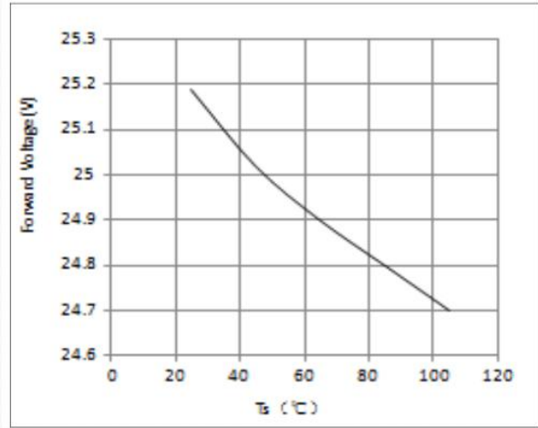
Fig 8. Ambient Temperature vs. Relative Forward Voltage
