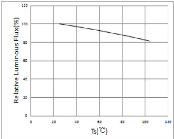
Fig 7. Ambient Temperature vs. Relative Luminous flux
