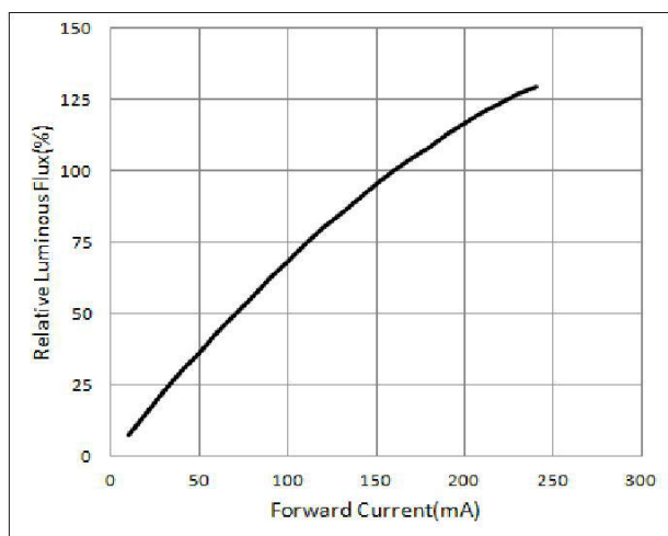
Fig 5. Forward Current vs. Relative Intensity, T_j = 25
