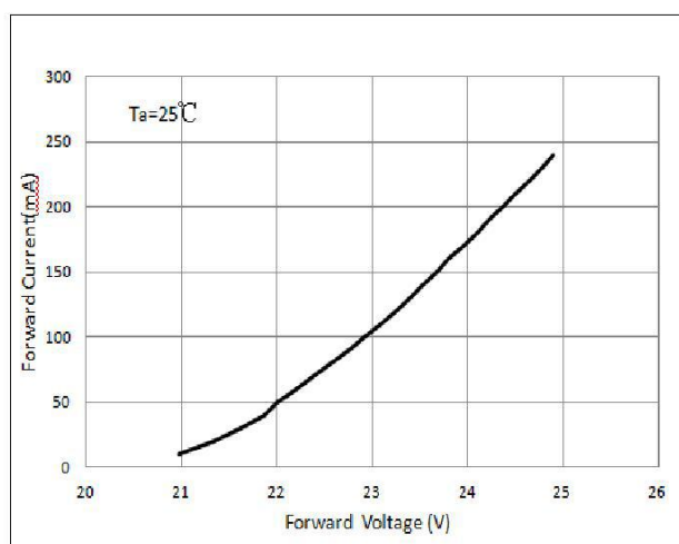
Fig 6. Forward Current vs. Forward Voltage, T_j = 25
